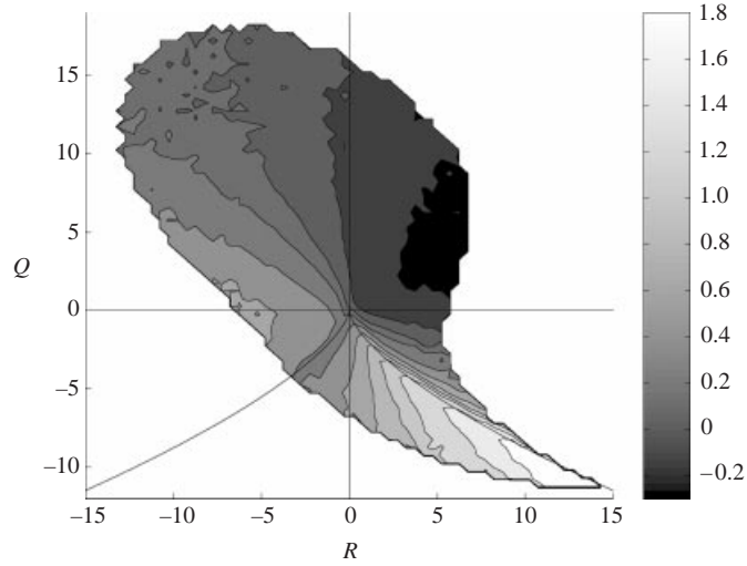
FIGURE 15. \langle -\mathcal{S}_i \lambda_i^2 | Q_A, R_A \rangle : the mean value of the production rate of g conditioned on the invariant Q_A and R_A obtained from run F . The scalar gradient is scaled with its mean value, the production rate is scaled with the mean strain rate and the invariants Q_A and R_A with (\frac{1}{2}\omega)^2 and (\frac{1}{2}\omega)^3 , respectively.
