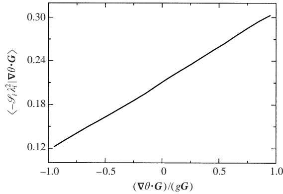
FIGURE 18. \langle -\mathcal{S}_i \lambda_i^2 | \nabla \theta \cdot \mathbf{G} / (g|\mathbf{G}|) \rangle : the mean value of the production term of g conditioned on the cosine of the angle between the scalar gradient and the imposed mean gradient. The statistics are obtained from run F .
