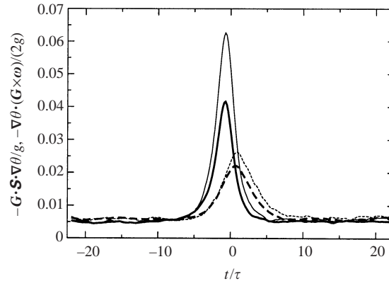
FIGURE 25. The time evolution of the production terms -\mathbf{G} \cdot \mathbf{S} \cdot \nabla \theta / g (solid lines) and -\nabla \theta \cdot (\mathbf{G} \times \boldsymbol{\omega}) / g (dashed lines) before and after g reaches a highest value at t = 0 . The time is normalized with the Kolmogorov time scale. This time evolution is an ensemble average of all events which satisfy g \geq 4\langle g \rangle (the thick lines) or g \geq 6\langle g \rangle (the thinner lines).
