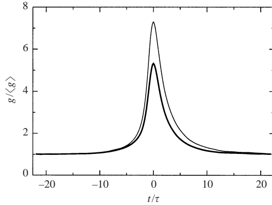
FIGURE 20. The time evolution of g in a short period of time before and after it reaches a high value. The time is normalized with the Kolmogorov time scale \tau and g with its mean value. This time evolution is an ensemble average of all events which satisfy g \geq 4\langle g \rangle (the thick line) or g \geq 6\langle g \rangle (the thinner line).
